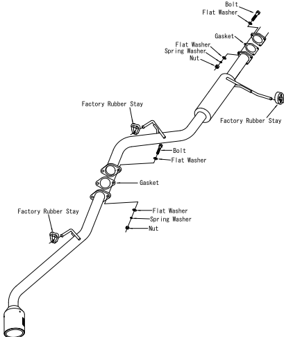
Muffler design
