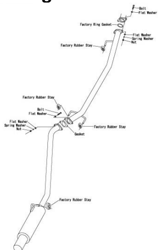
Muffler design
