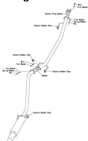
Muffler design
